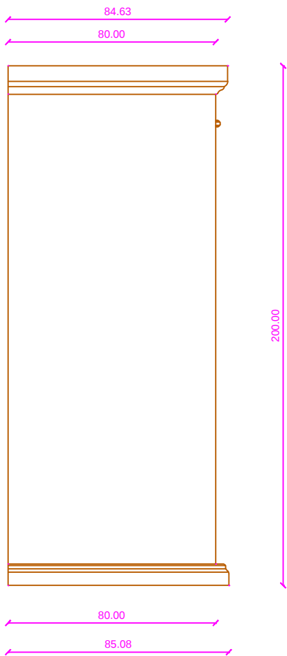
SIDE ELEVATION
