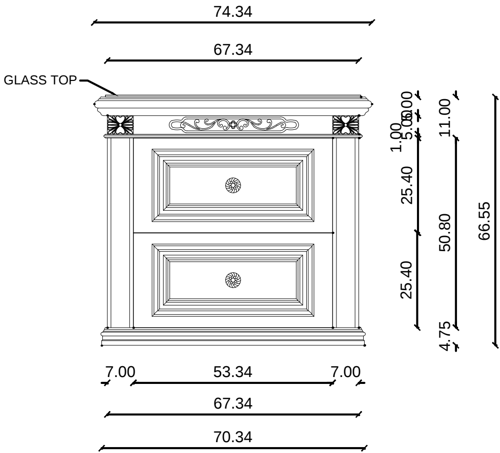
FRONT ELEVATION
