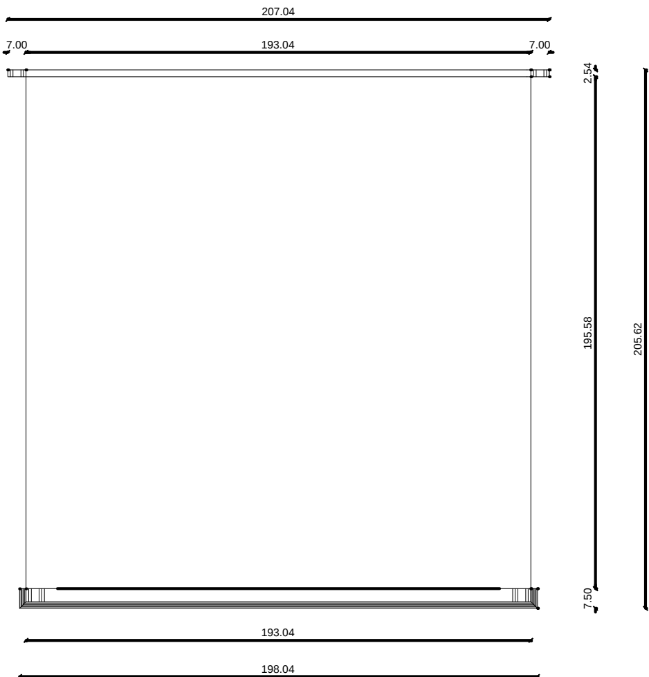
PLAN
