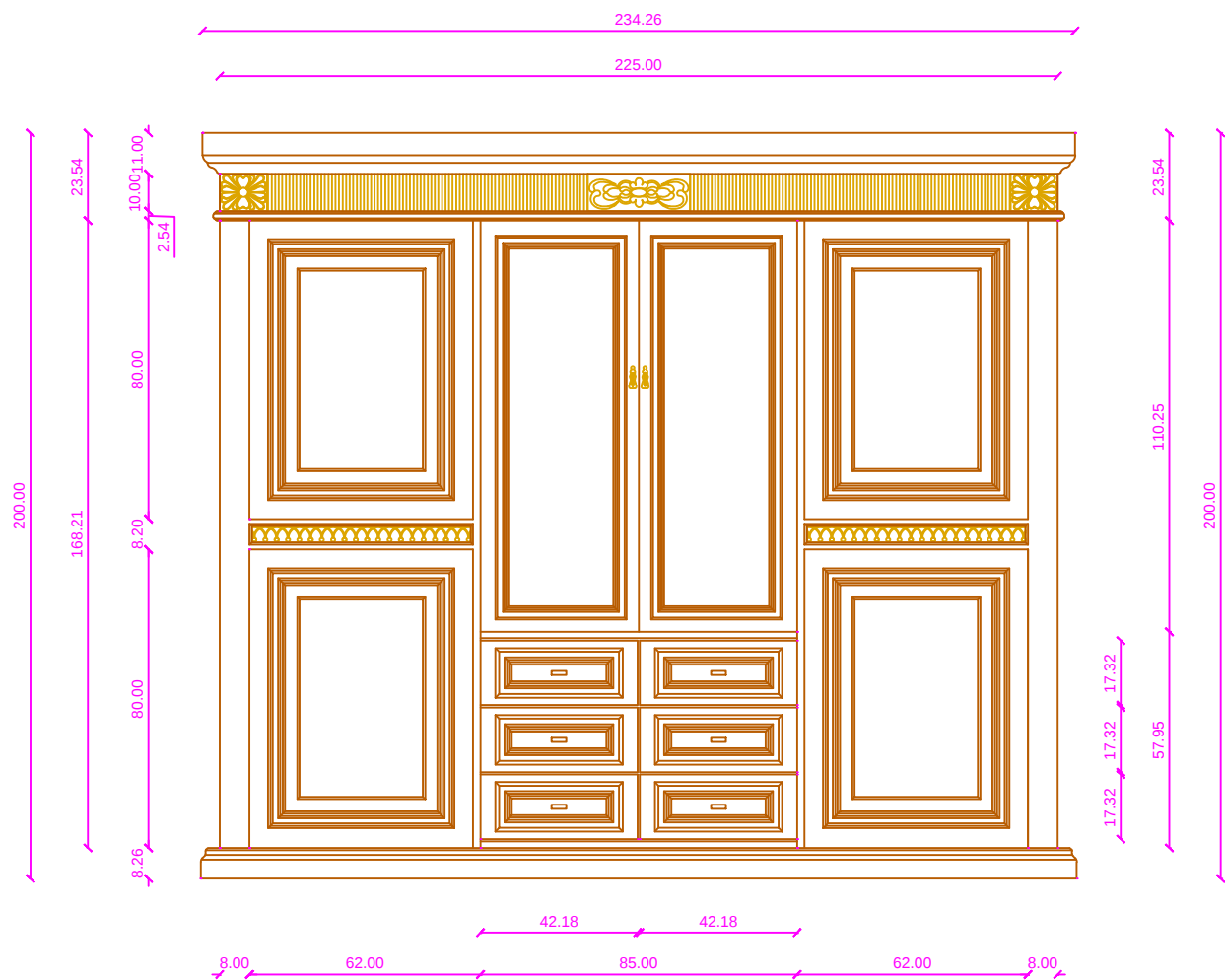
FRONT ELEVATION
